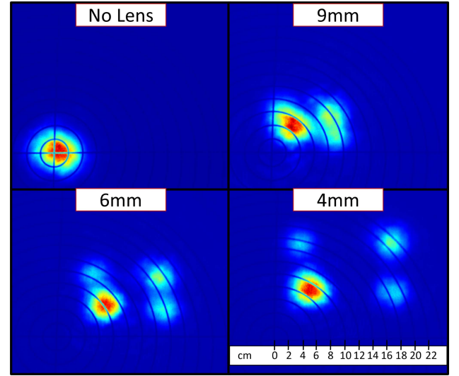
Fig. 11. Measured angular steering range for the focal lengths of 4 mm, 6 mm, and 9 mm, with four beams active at the same time (the rings are spaced 2 cm apart).
